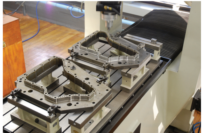
Automotive Punches
